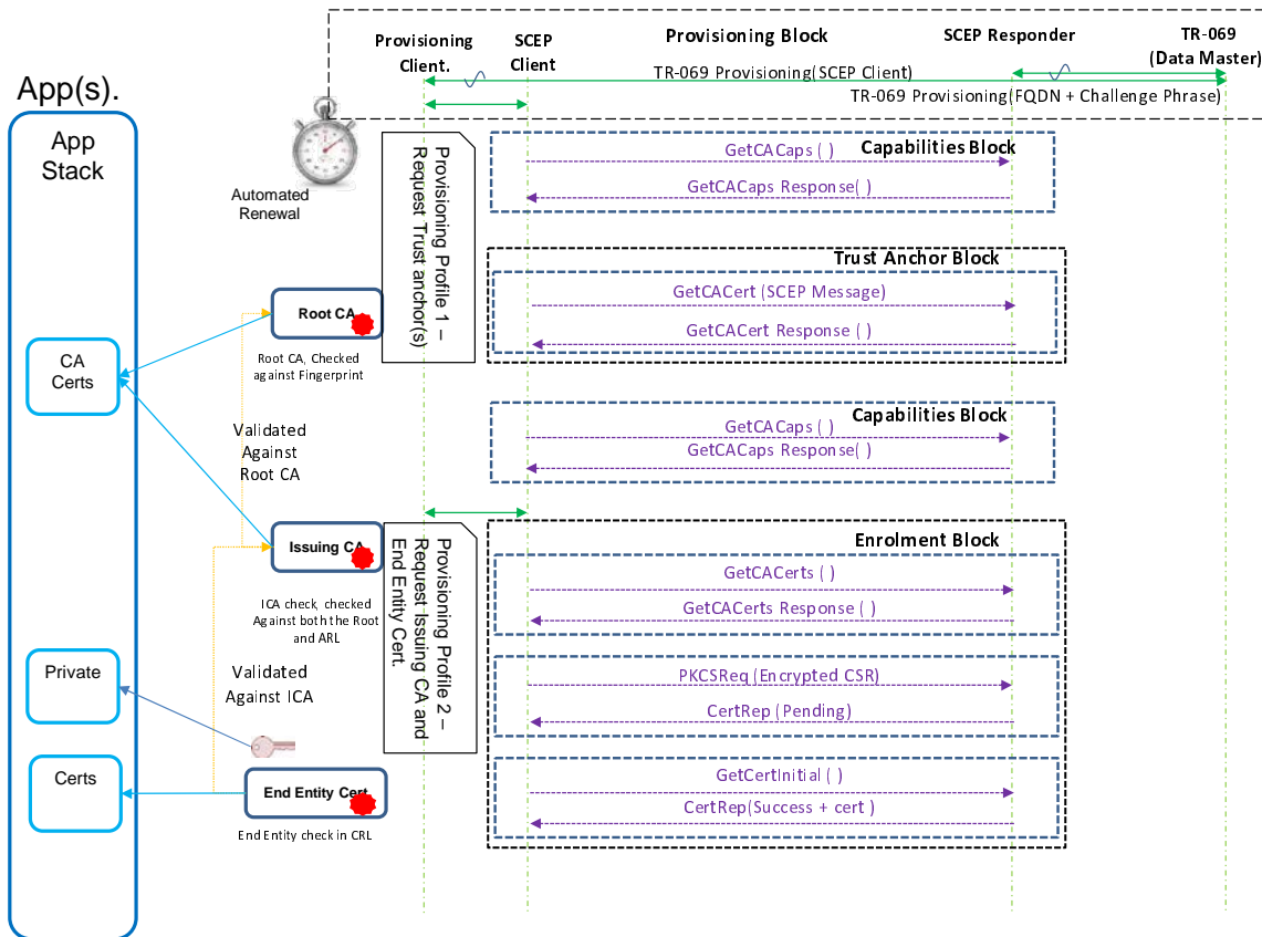
Figure L.1: SCEP certificate provisioning procedure
