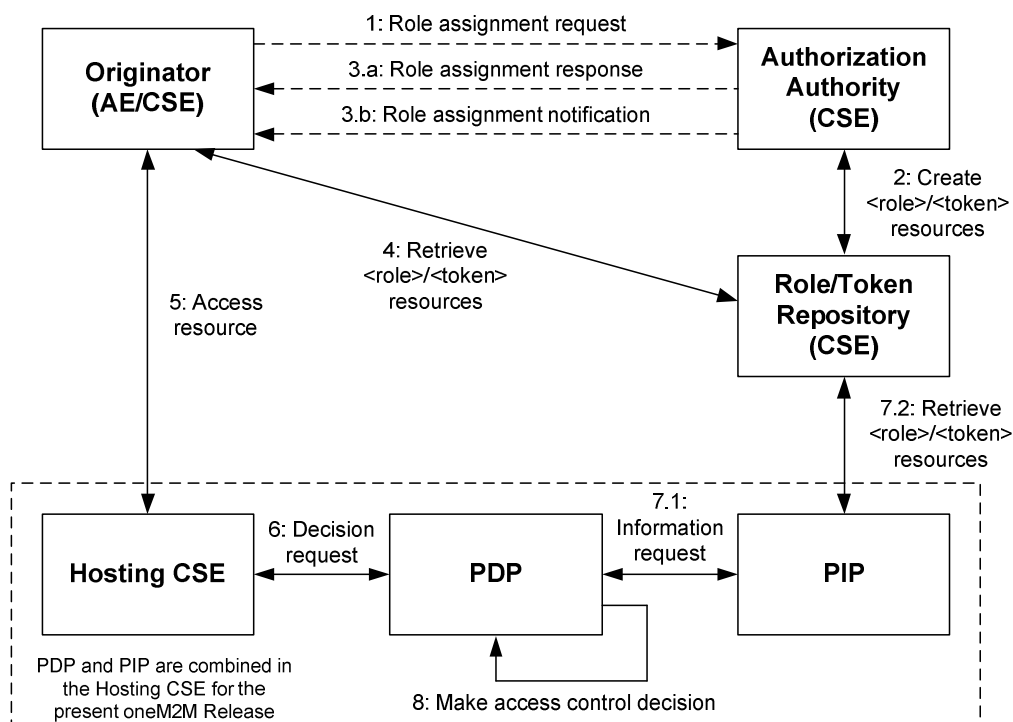
Figure 7.4.1-1: Role based access control architecture
