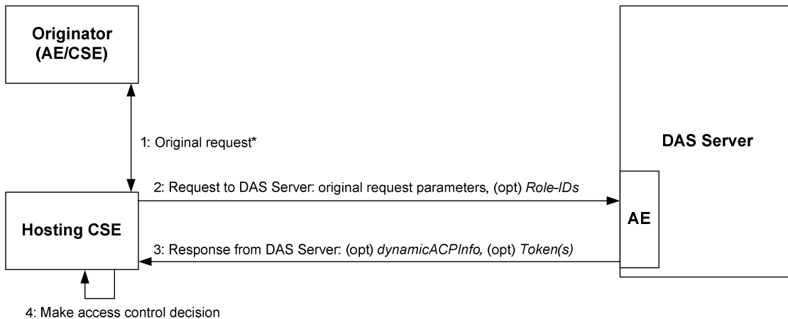
Figure 7.3.2.1-2: Direct Dynamic Authorization
