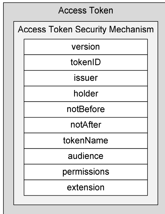
Figure 7.3.2.4-1: Structure of token
